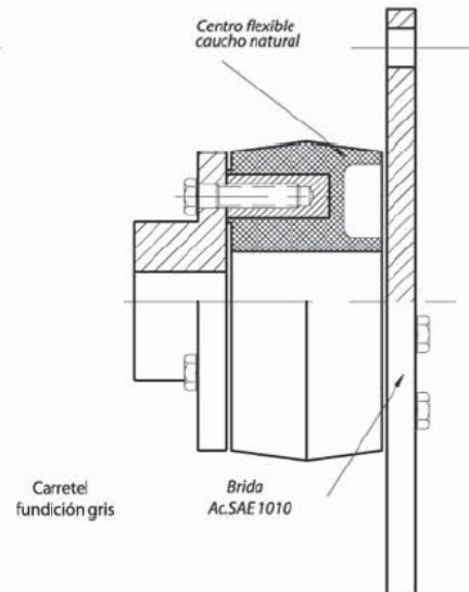
VERSION BRIDA
