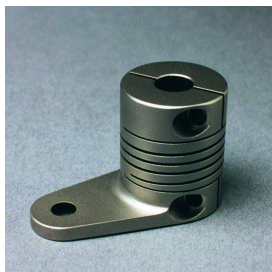
Integrating a lever arm into a clamp attachment flexure allowed linear motion to be converted to rotary motion.
