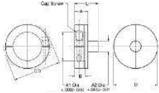
Sample part number: AH250-52-20. Material: Aluminum Alloy.
