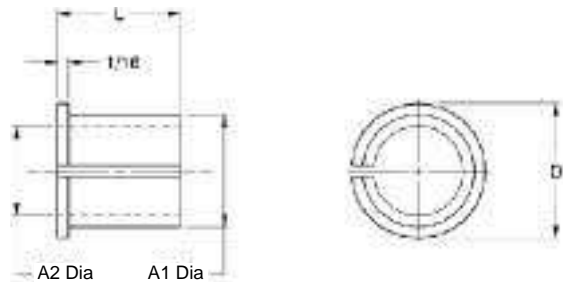
Sample part number: BR075-20-16. Material: Aluminum Alloy.
