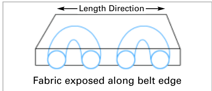
No longitudinal fibers exposed at belt edges. No fraying.
