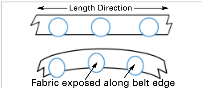
This design provides increased flexibility for knife edge transfers.
