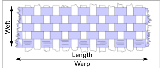
Weave pattern in traditional multi x mono belts.
