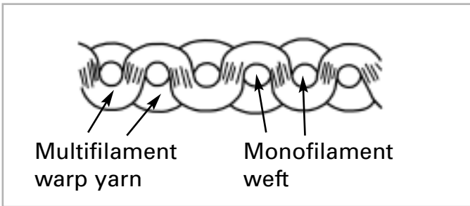
Longitudinal multifilament fibers exposed at belt edges.
