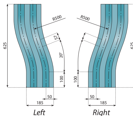
Compact Version (view from above)
