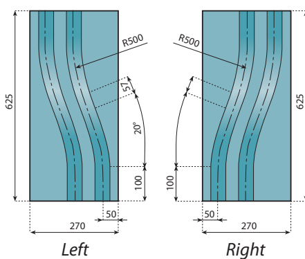
Standard Version (view from above)
