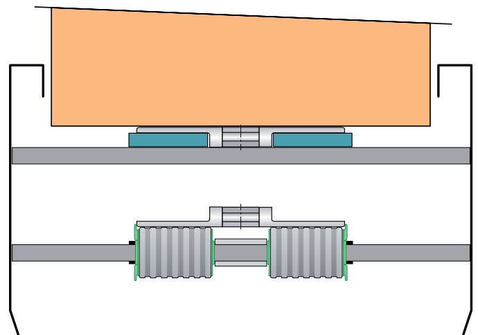
Principle sketch of a possible construction.
