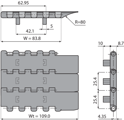
Single track version or,
