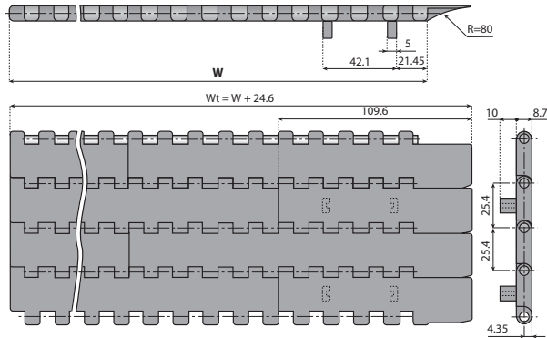
Connected to full width belt
