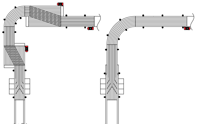
conventional layout
