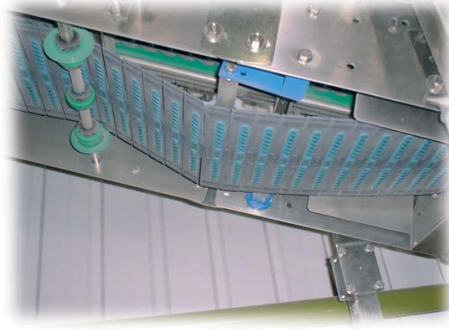
Common tensioner
